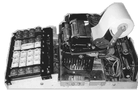
BUSICOM Calculator, Engineering Prototype, 1971, Credit: Gift of Federico Faggin
